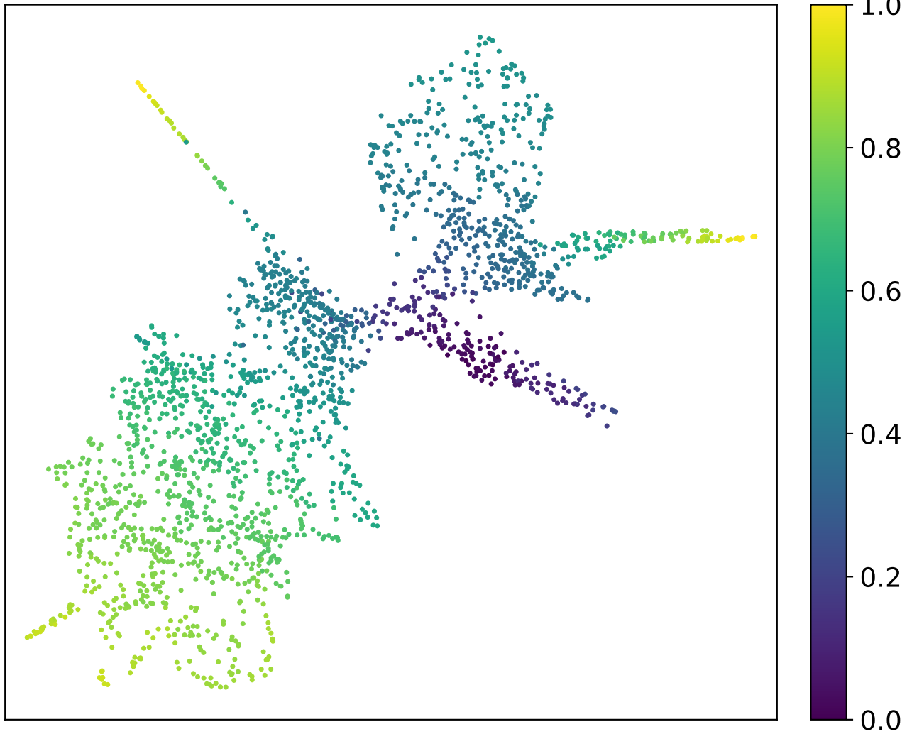
Randers SMACOF alpha=0: lineage pseudotime
