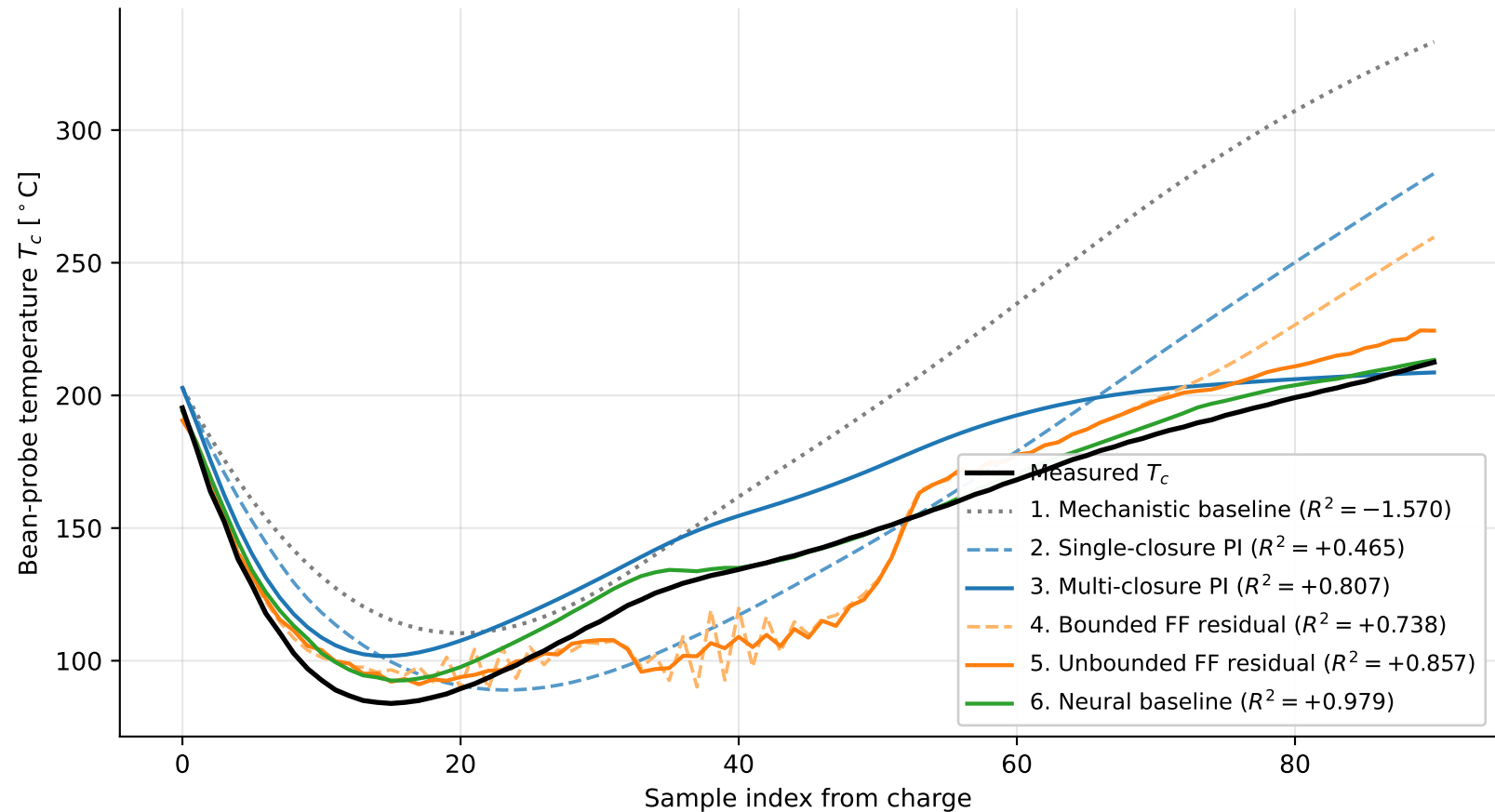
Representative held-out rollout (test roast, seed 11): ROAST_160_P13
