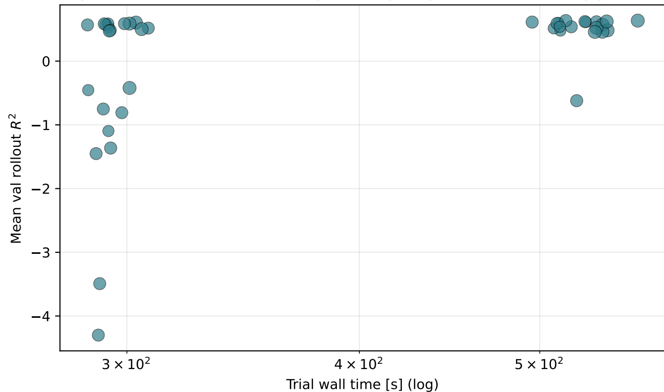
Physics Informed Model — compute vs quality (marker size \propto \log params)
