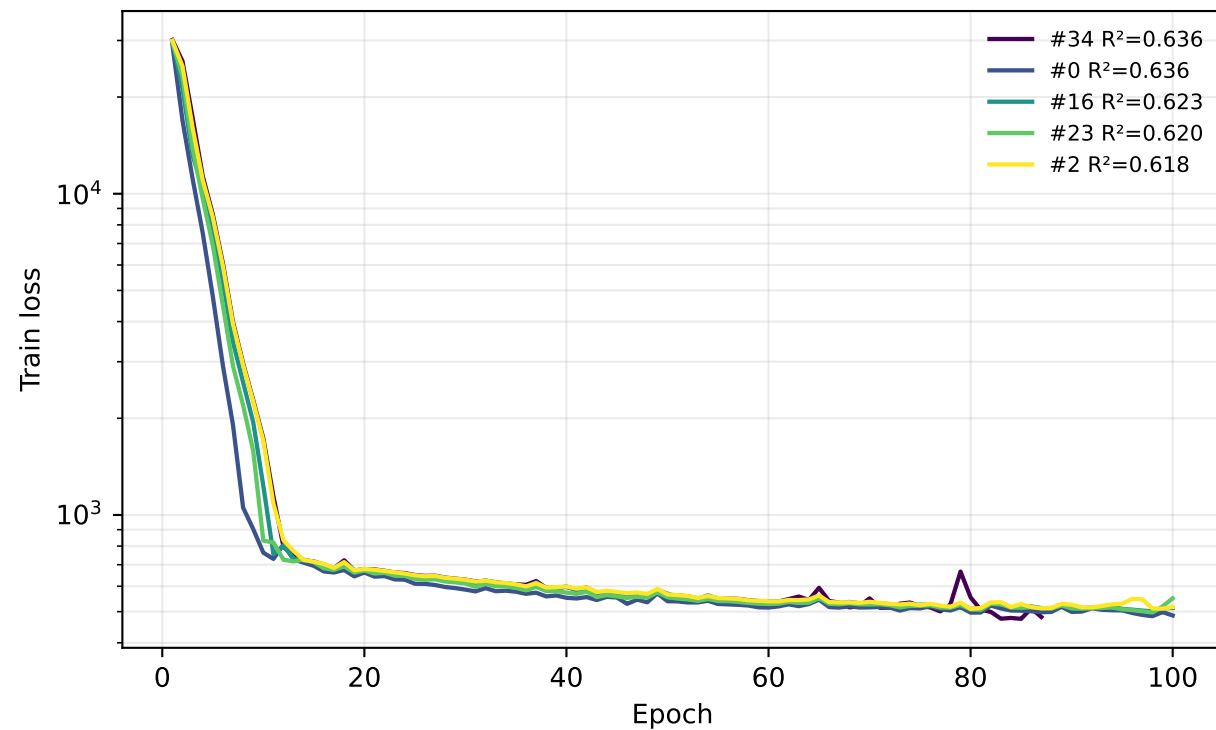
Train loss
