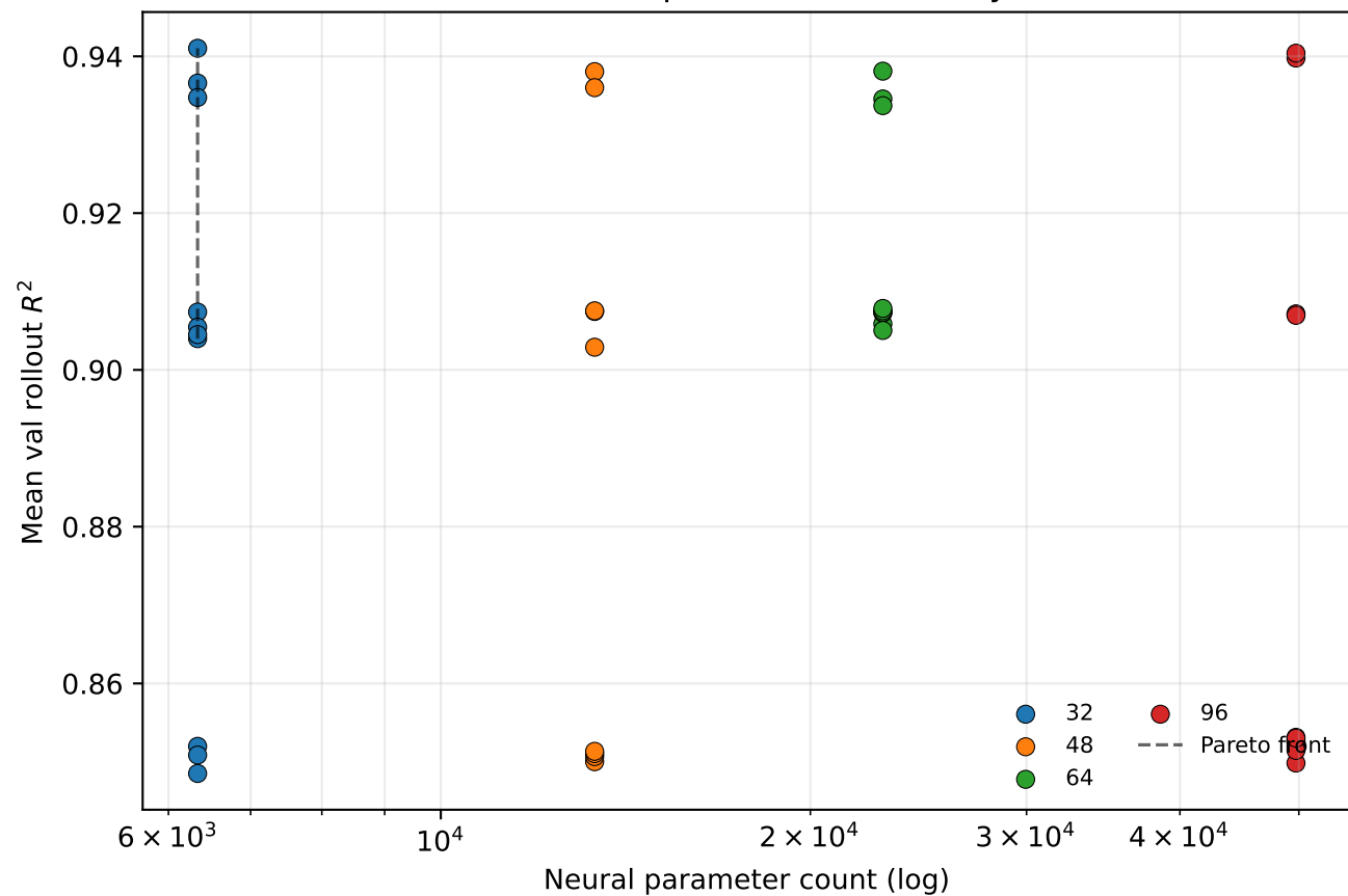
Residual LSTM — parameter efficiency Pareto
