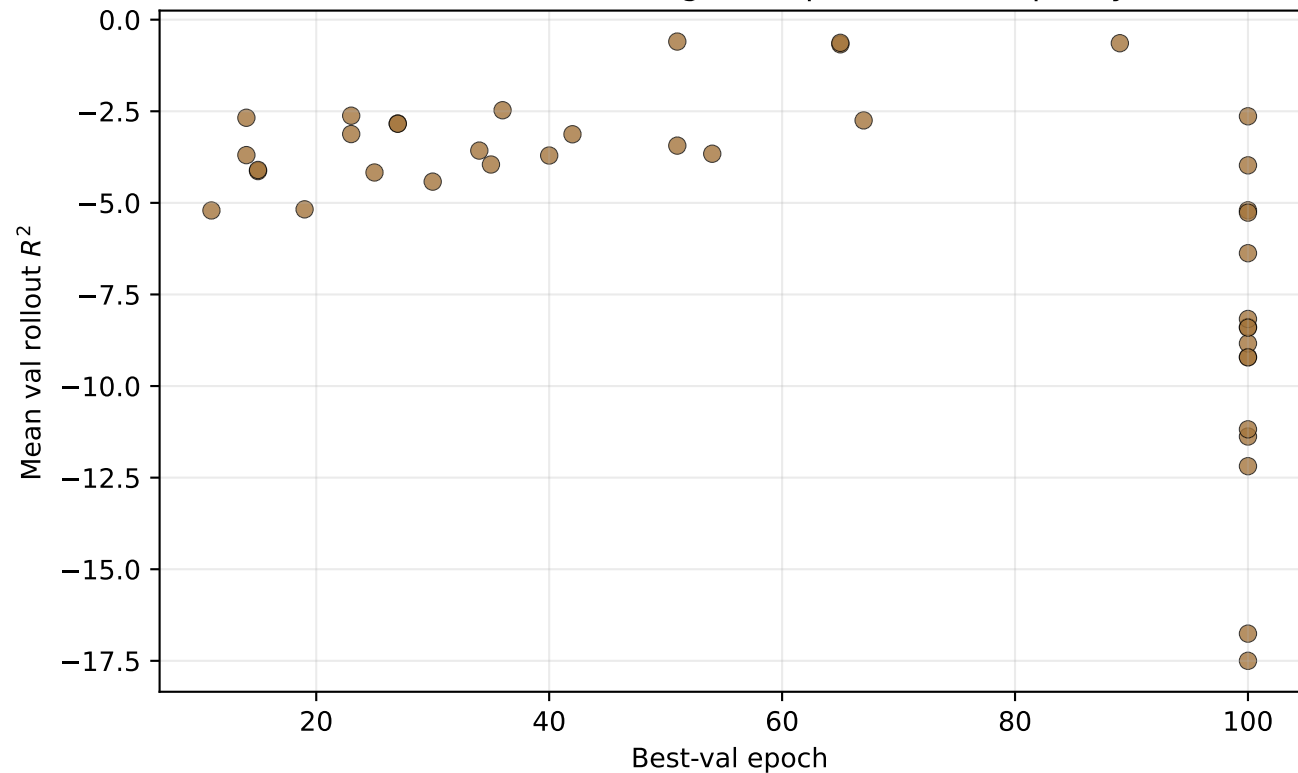
Mechanistic — convergence speed vs final quality
