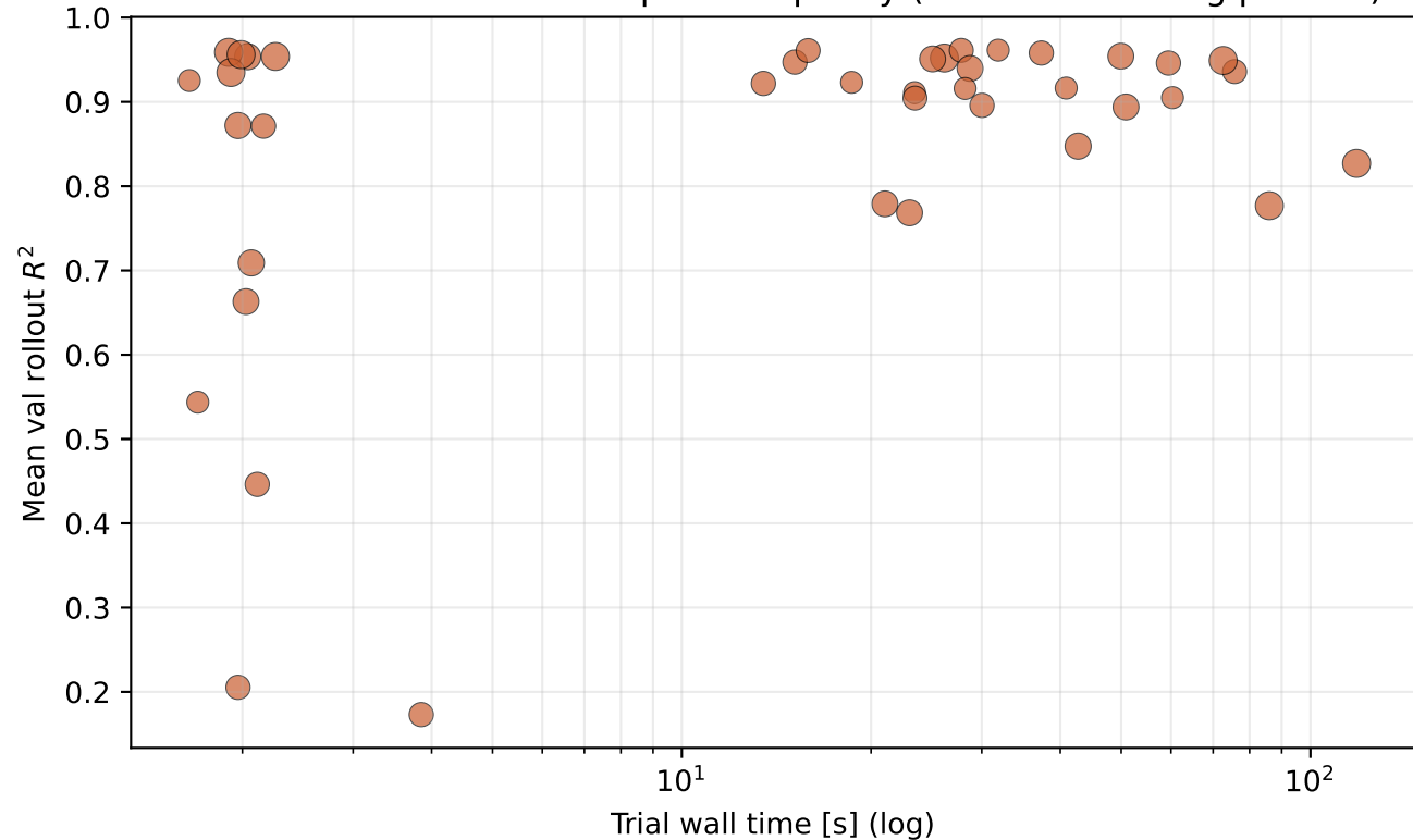
Neural Net Baseline — compute vs quality (marker size \propto \log params)
