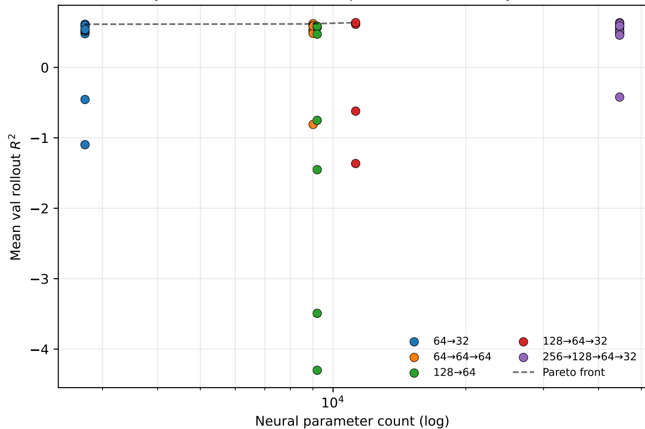
Physics Informed Model — parameter efficiency Pareto
