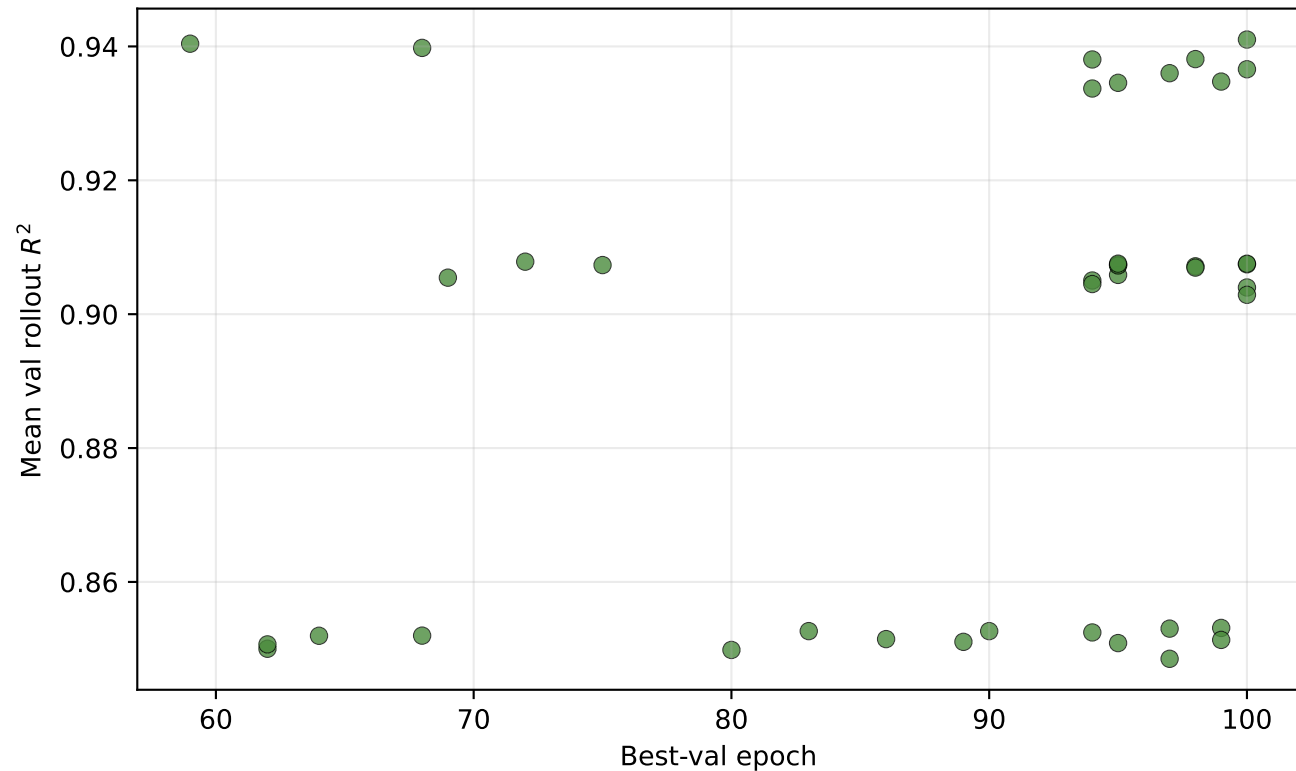
Residual LSTM — convergence speed vs final quality
