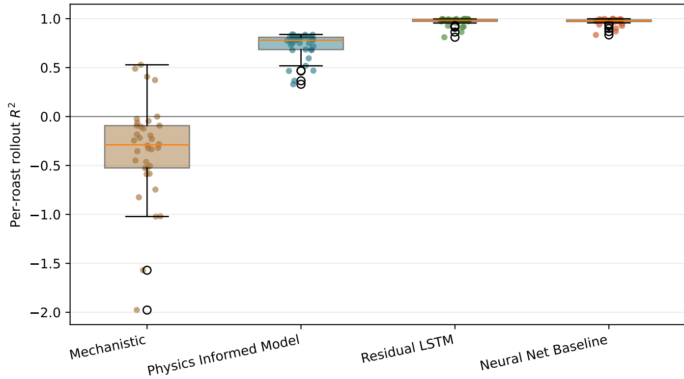
Held-out per-roast rollout R^2 (seed 11, HPO sweep)
