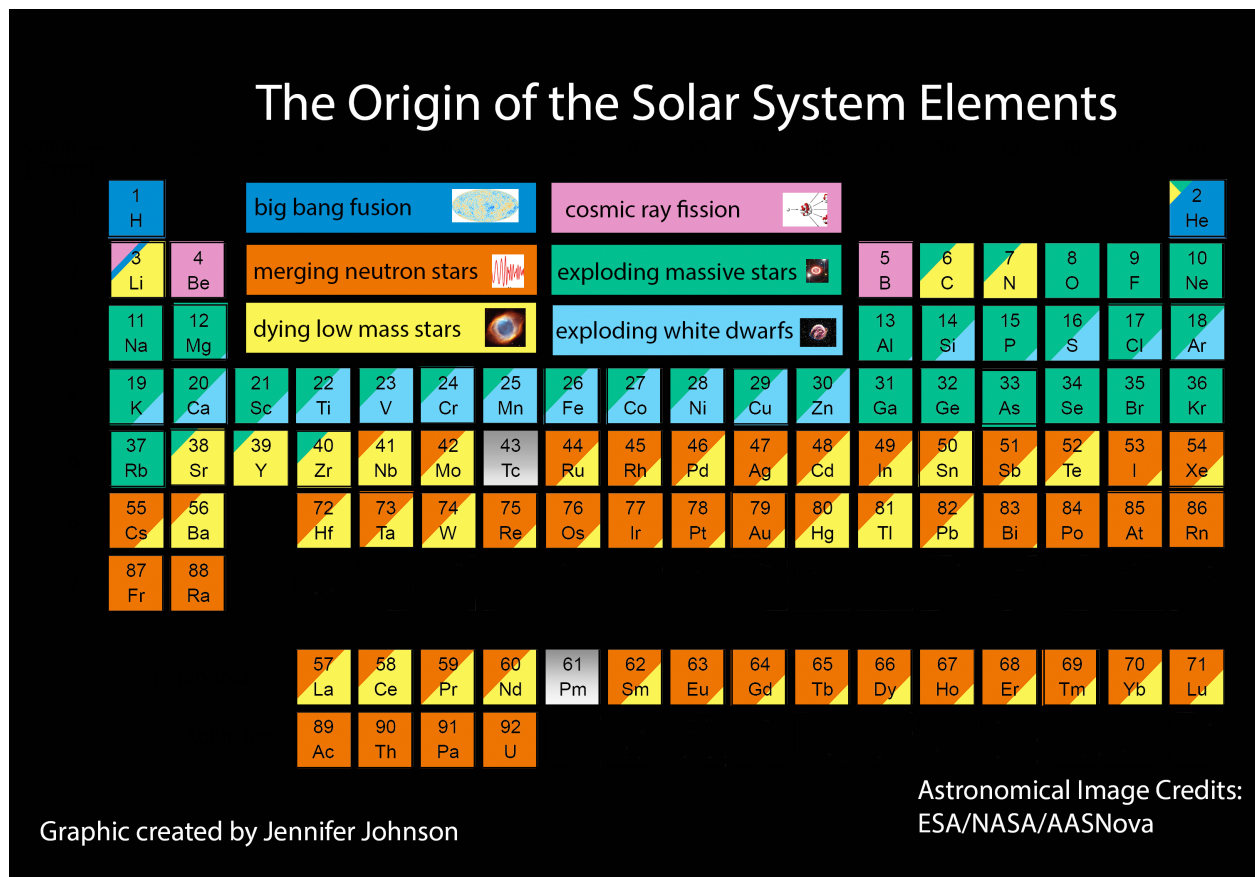
Figure 1.1: Taken from Johnson (2017) : Periodic table shaded according to the origin of the elements in the solar system.
