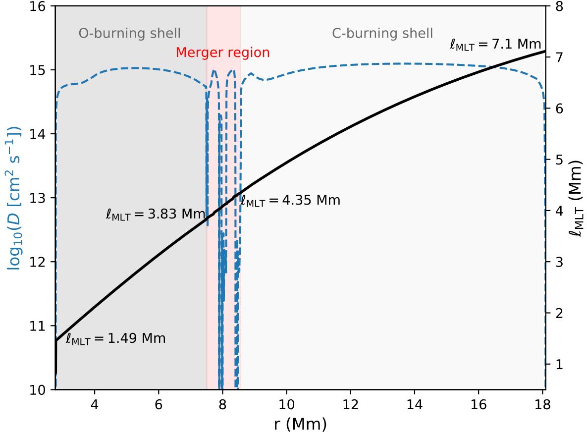
Figure 1.5: O- and C-burning shells in the 15M_{\odot} Z = 0.02 model from Ritter et al. (2018b) at model number 9200 right before the merger with the C-shell is fully realized. The left y-axis shows the diffusion coefficient in blue, and the right y-axis shows the mixing length in black. The O-shell is from 2.79\text{--}7.49 \times 10^6 m, the merger region is from 7.49\text{--}8.56 \times 10^6 m, and the C-burning shell is from 8.56\text{--}18 \times 10^6 m.
