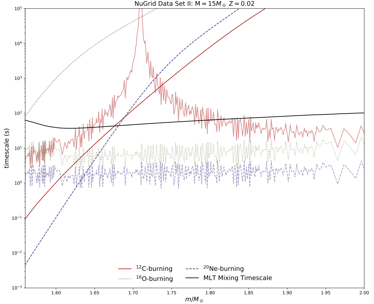
Figure 1.3: Timescales of mixing and burning during the O-C shell merger of a 15M_{\odot} Z = 0.02 stellar model from Ritter et al. (2018b) at model number 9200. The black line show the timescale from MLT mixing. The solid red line shows the timescale for a variety of ^{12}\text{C} burning reactions and the jagged red line is its corresponding reaction scale height timescale. The dotted green line shows the timescale for a variety of ^{16}\text{O} burning reactions and the jagged green line is its corresponding reaction scale height timescale. The dashed blue line shows the timescale for a variety of ^{20}\text{Ne} burning reactions and the jagged blue line is its corresponding reaction scale height timescale.
