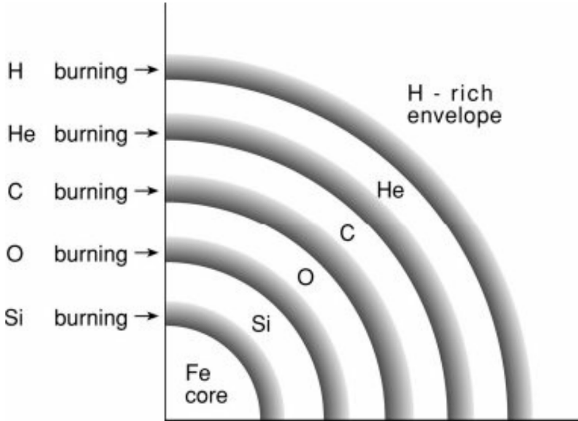
Figure 1.1: Taken from Priyalnik (2009) Figure 9.19: Schematic structure of a supernova progenitor star.
