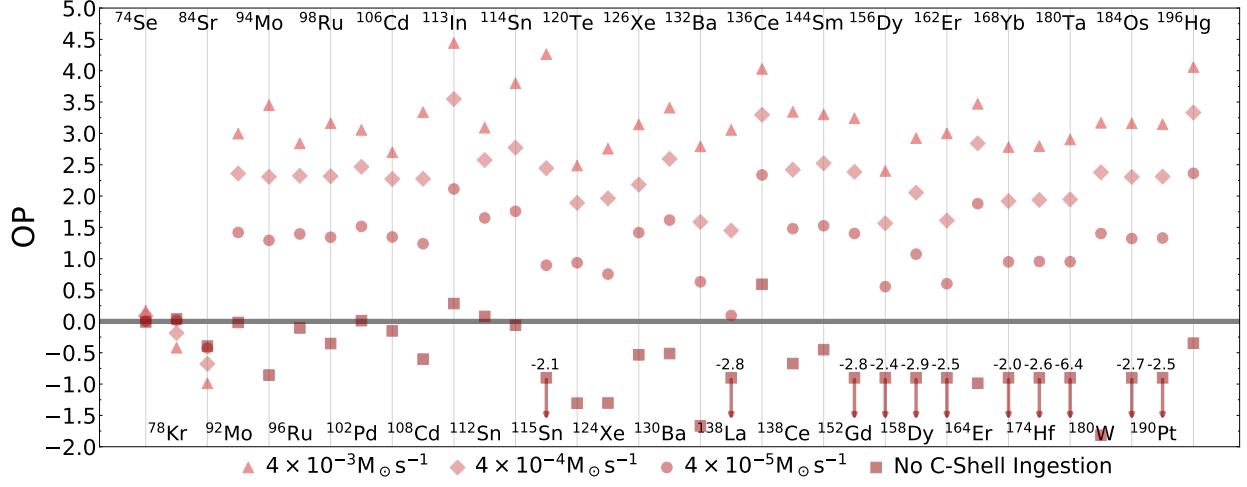
Figure 2.18: The overproduction compared to initial of the p nuclei for the 10 \times 3D -inspired mixing scenario for no ingestion, 4 \times 10^{-5} M_{\odot} \text{s}^{-1} , 4 \times 10^{-4} M_{\odot} \text{s}^{-1} , and 4 \times 10^{-3} M_{\odot} \text{s}^{-1} . Arrows denote OP_{\text{out}} of bounds and the true OP_{\text{in}} is written above. The average spread in production OP_{\text{max}} - OP_{\text{min}} = 1.78 dex excluding the no ingestion case. OP = 0 is the initial amount.
