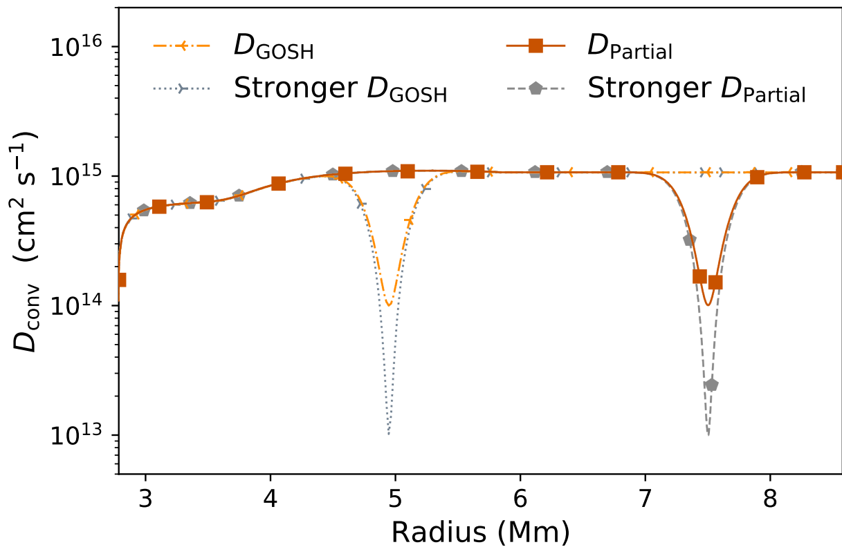
Figure 2.5: The quenched mixing scenario convective profiles. The dashed light orange line and dotted light grey line are the GOSH-like profiles with a dip centred at r = 4.95\text{Mm} . The solid red line and dashed dark grey line are the partial merger profiles with a dip centred r = 7.5\text{Mm} . The MLT profile is omitted for clarity.
