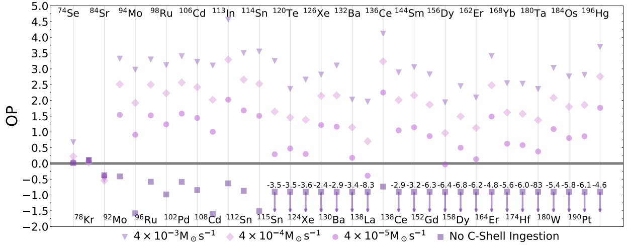
Figure 2.19: The overproduction compared to initial of the p nuclei for the 50 \times 3D -inspired mixing scenario for no ingestion, 4 \times 10^{-5} M_{\odot} \text{s}^{-1} , 4 \times 10^{-4} M_{\odot} \text{s}^{-1} , and 4 \times 10^{-3} M_{\odot} \text{s}^{-1} . Arrows denote OP_{\text{out}} of bounds and the true OP_{\text{in}} is written above. The average spread in production OP_{\text{max}} - OP_{\text{min}} = 1.84 dex excluding the no ingestion case. OP = 0 is the initial amount.
