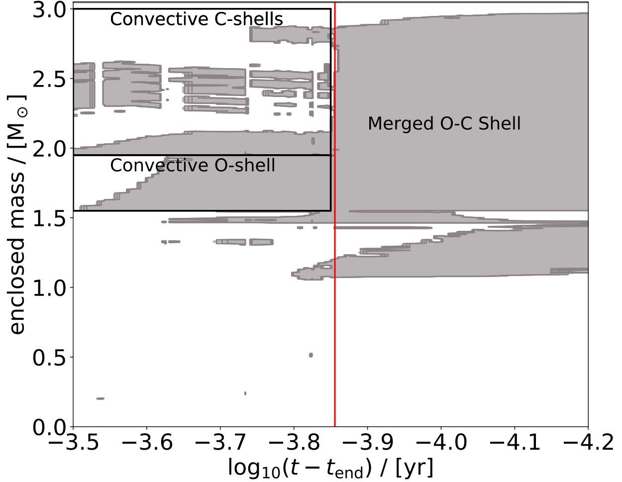
Figure 1.2: Kippenhahn diagram showing the merger of the convective O and C-burning shells for the 15 M_{\odot} Z = 0.02 model from Ritter et al. (2018b) . The O-burning shell extends from 1.55\text{--}1.95 M_{\odot} . The first convective C-burning shell sits directly on top from 1.96\text{--}2.11 M_{\odot} and additional convective C-burning shells that are ingested are above. The merger onsets at \log_{10}(t - t_{\text{end}})/\text{yr} \approx -3.85 and reaches full extent at \approx -4 .
