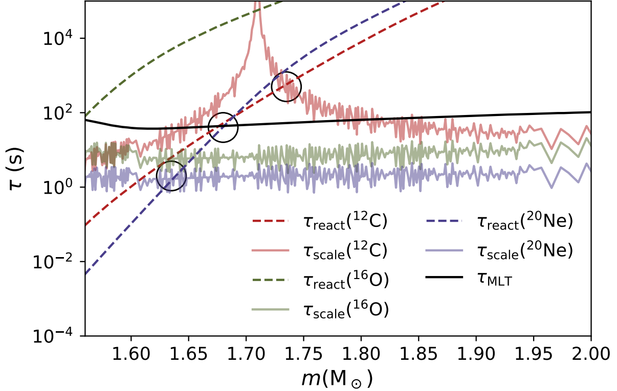
Figure 1.6: Timescales \tau_{\text{MLT}} , \tau_{\text{react}} , and \tau_{\text{scale}} vs mass for the 15 M_\odot Z = 0.02 stellar model from Ritter et al. (2018b) during the merger at \log_{10}(t - t_{\text{end}}) \approx -3.88 . The black line is \tau_{\text{MLT}} . The dashed red line is \tau_{\text{react}} for ^{12}\text{C} , and the solid red line is \tau_{\text{scale}} for ^{12}\text{C} . Likewise, the green lines are for ^{16}\text{O} , and the purple lines are for ^{20}\text{Ne} . Black circles are provided where D_\alpha = 1 for ^{12}\text{C} and ^{20}\text{Ne} .
