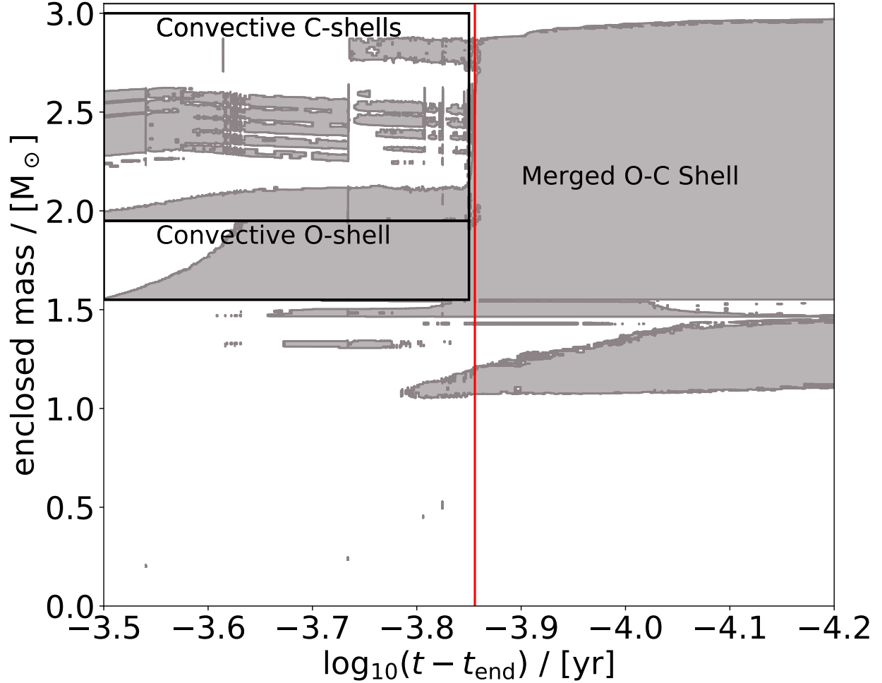
Figure 1.5: Zoom in view of Figure 1.3 showing the merger of the convective O and C-burning shells for the 15 M_{\odot} Z = 0.02 model from Ritter et al. (2018b). The O-burning shell extends from 1.55\text{--}1.95 M_{\odot} . The first convective C-burning shell sits directly on top from 1.96\text{--}2.11 M_{\odot} and additional convective C-burning shells that are ingested are above. The merger onsets at \log_{10}(t - t_{\text{end}})/\text{yr} \approx -3.85 and reaches full extent at \approx -4 .
