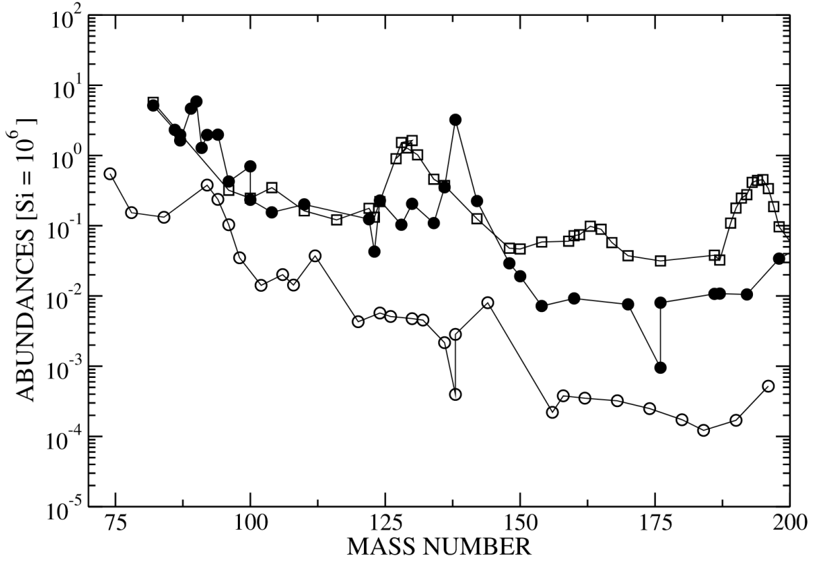
Figure 1.4: Taken from Rapp et al. (2006) : Abundance distribution of heavy isotopes that can be entirely ascribed to s process (filled circles), r process (squares), and p process (open circles) nucleosynthesis.
