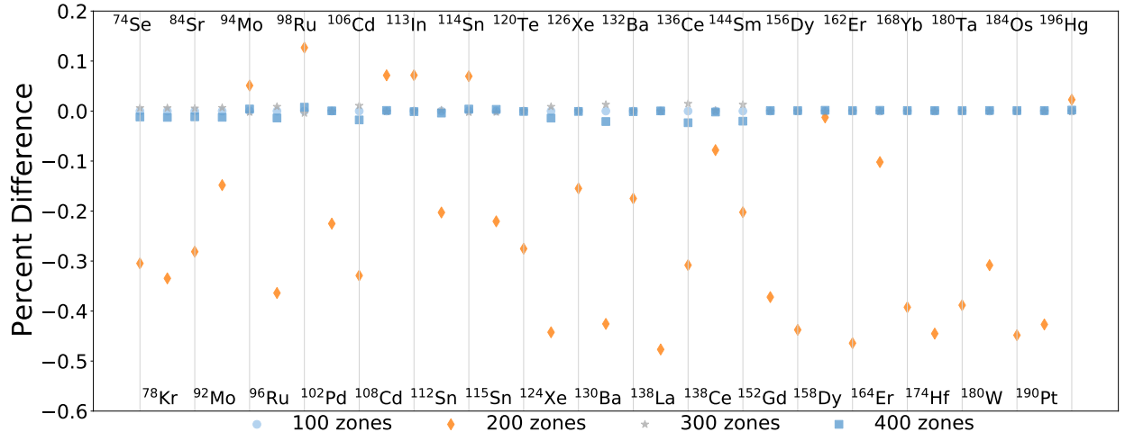
Figure 1.8: Mass resolution test for the p nuclei using a post-processed model of the 15 M_{\odot} Z = 0.02 stellar model from Ritter et al. (2018b) at 110 s of ingestion and 400 mass zones. Percent difference is calculated as the (\text{case} - 100 \text{ zones}) / (100 \text{ zones}) . The 100 zones case has a percent difference of 0%.
