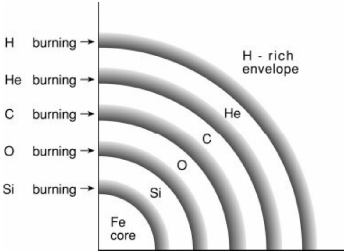
Figure 1.2: Taken from Priyalnik (2009) Figure 9.19: Schematic structure of a supernova progenitor star. The Ne-burning layer is not shown but would be between the C- and O-layers.
