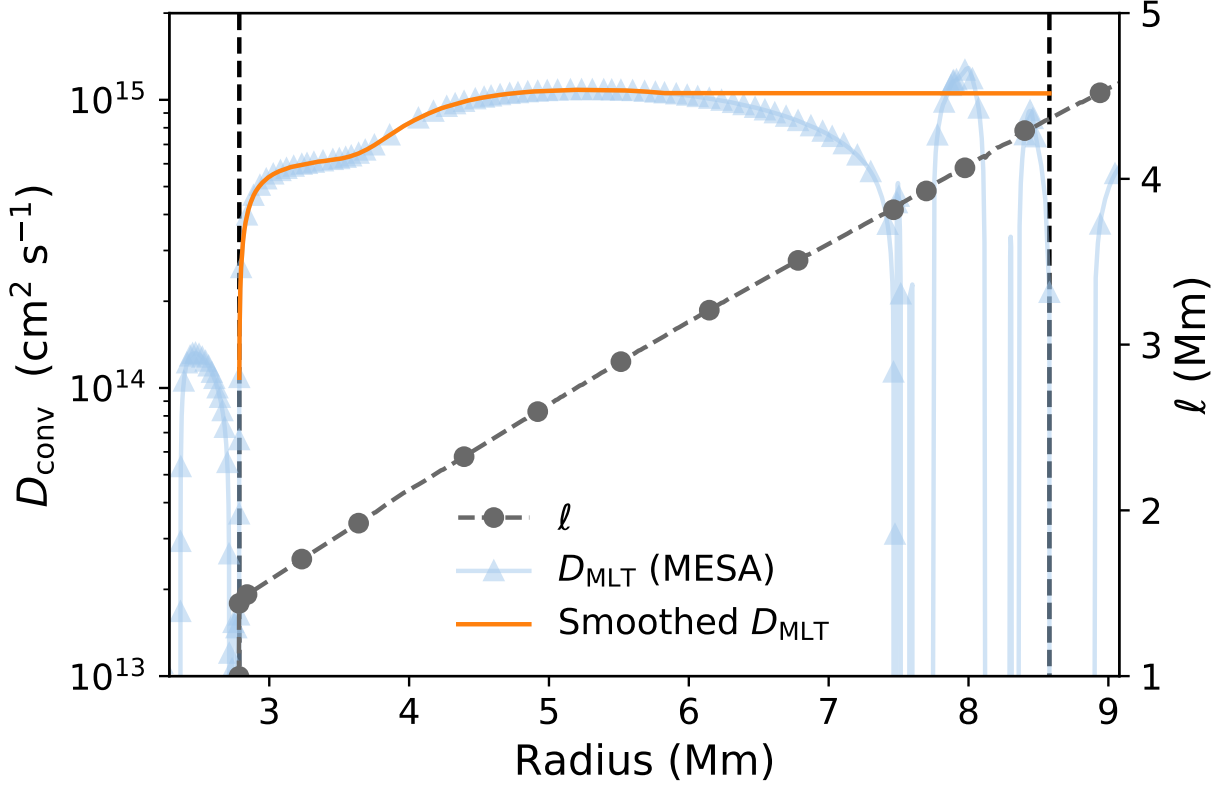
Figure 2.3: The diffusion coefficient profile and mixing length at model number 9200 for the M_{\text{ZAMS}} = 15M_{\odot} , Z = 0.02 model. The light blue line is D from MESA, the orange line the smoothed D used for the MLT mixing scenario in this paper, and the grey line is the mixing length. Black dashed lines mark the shell boundaries for this paper.
