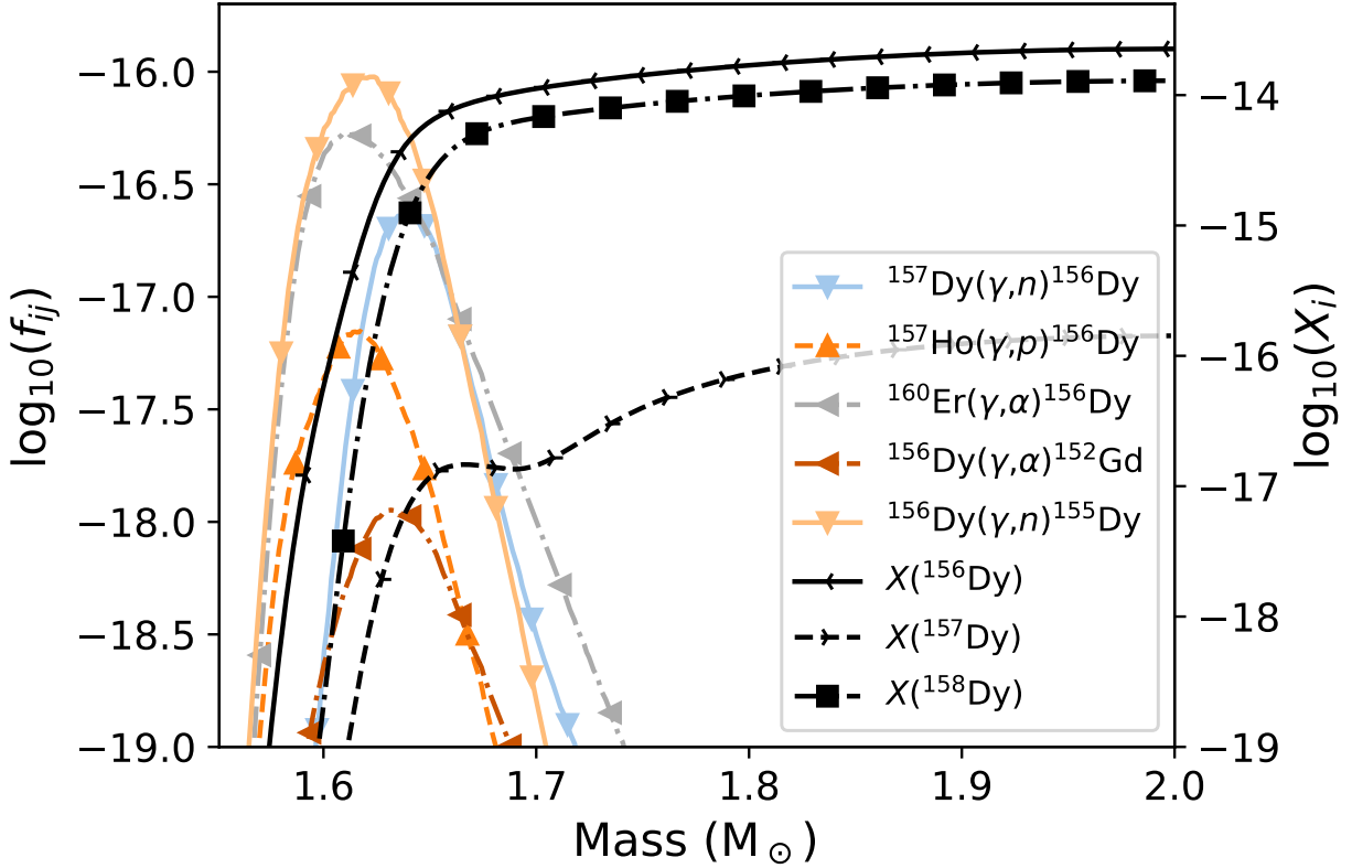
Figure 2.7: Reaction fluxes f_{ij} for ^{156}\text{Dy} and mass fractions X_i for ^{156-158}\text{Dy} without radiogenic contributions for the MLT scenario with no ingestion after t = 110\text{s} . The direction of reactions i \rightarrow j are written as left to right in the legend.
