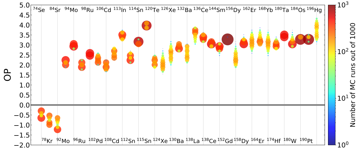
Figure 2.20: Histogram showing the spread due to varying (\gamma, p) , (\gamma, n) , (\gamma, \alpha) and corresponding capture rates for unstable n -deficient isotopes from Se–Po for the 3D-inspired mixing scenario. Colour and size both correspond to the logarithmic binning of Monte Carlo runs. The average spread \text{OP}_{\text{max}} - \text{OP}_{\text{min}} = 0.59 dex. \text{OP} = 0 is the initial amount.
