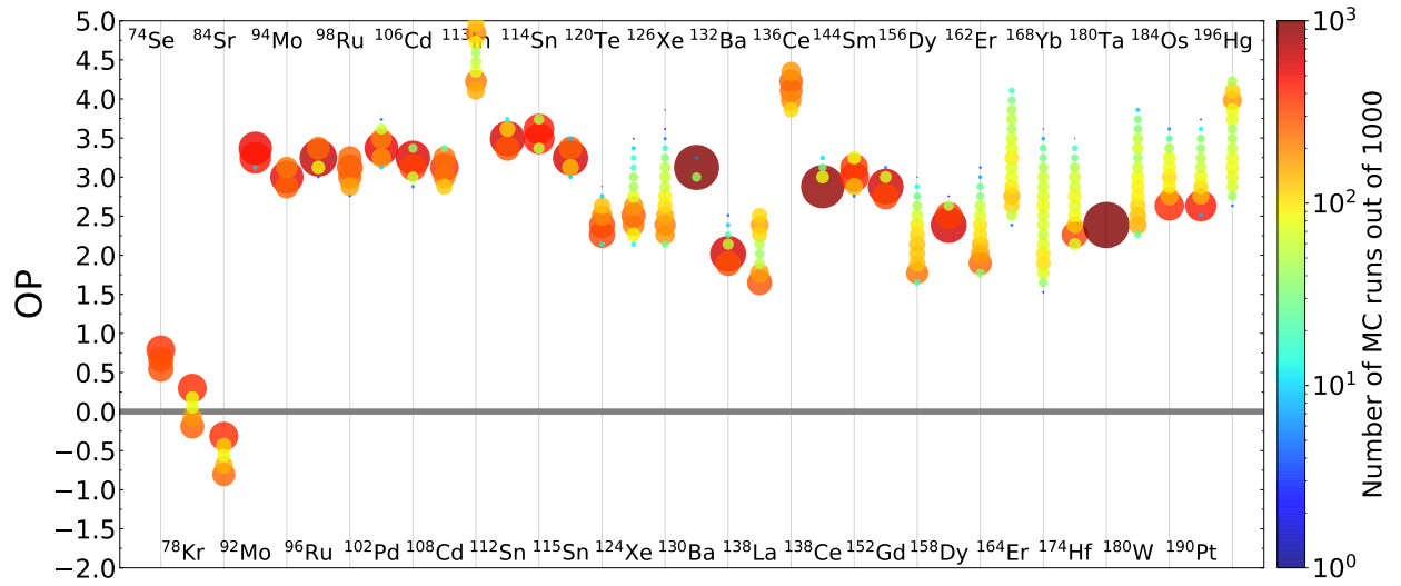
Figure 2.23: Histogram showing the spread due to varying (\gamma, p) , (\gamma, n) , (\gamma, \alpha) and corresponding capture rates for unstable n -deficient isotopes from Se–Po for the 50 \times 3\text{D} -inspired mixing scenario. Colour and size both correspond to the logarithmic binning of Monte Carlo runs. The average spread \text{OP}_{\text{max}} - \text{OP}_{\text{min}} = 0.79 dex. \text{OP} = 0 is the initial amount.
