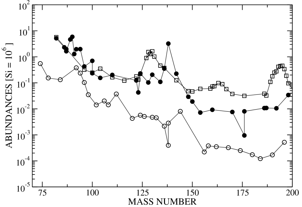
Figure 1.5: Taken from Rapp et al. (2006) : Abundance distribution of heavy isotopes that can be entirely ascribed to s process (filled circles), r process (squares), and p process (open circles) nucleosynthesis.
