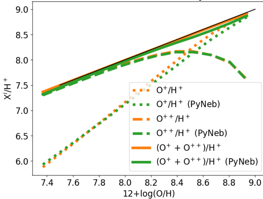
Ionic abundances from model and from PyNeb (direct method)
