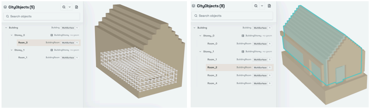
Figure 3: Result of the voxel-based surface extraction (Section 4.4.2) for the House. Left: at voxel size 0.5m, the output again contains 5 CityObjects, matching the two real rooms. Right: at 0.25m, three additional rooms appear; there are now rooms that are not real rooms but the gap inside the exterior wall between its inner and outer layer.
