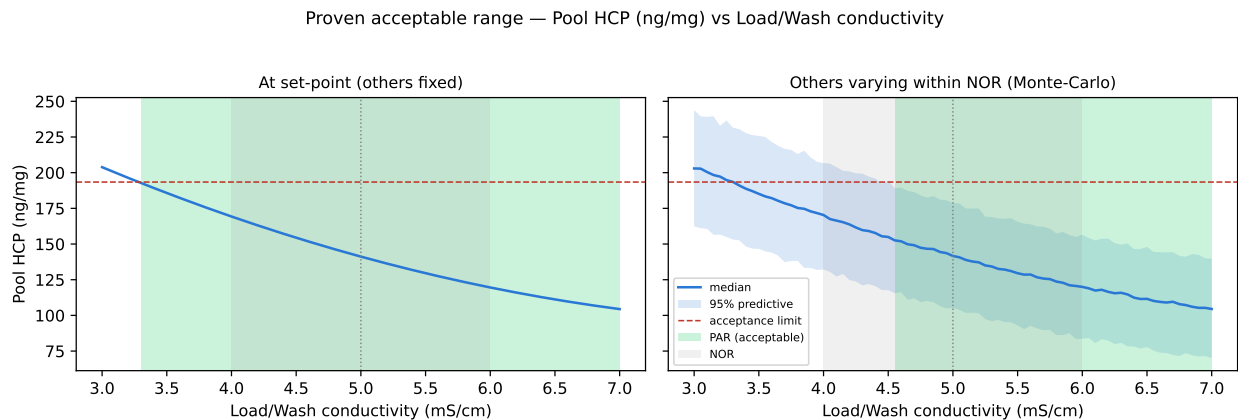
Figure 7.2: Pool host cell protein against load/wash conductivity, analysed against the in-process limit for this step. The acceptable region is shaded green. The limit is the pool concentration from which anion exchange can still reach the drug substance criterion, divided by an assurance margin.
