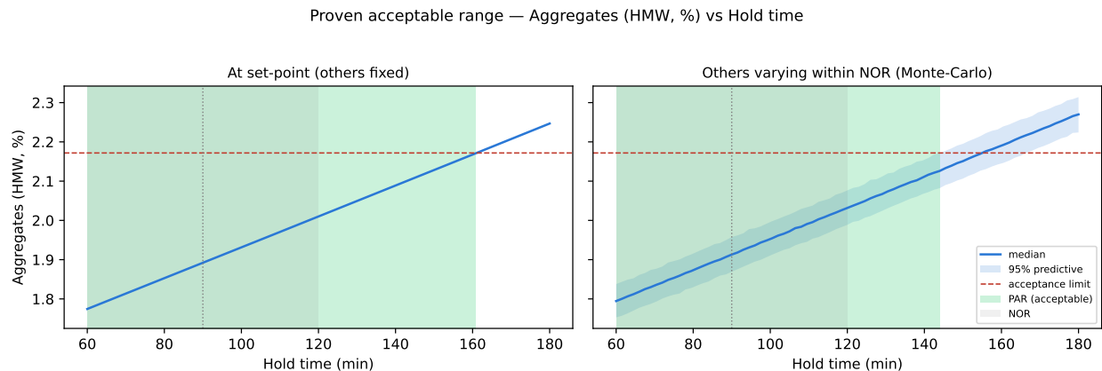
Figure 7.2: Proven acceptable range for pool aggregate against hold time, at set-point (left) and with the other parameters propagated across their normal operating ranges (right).
