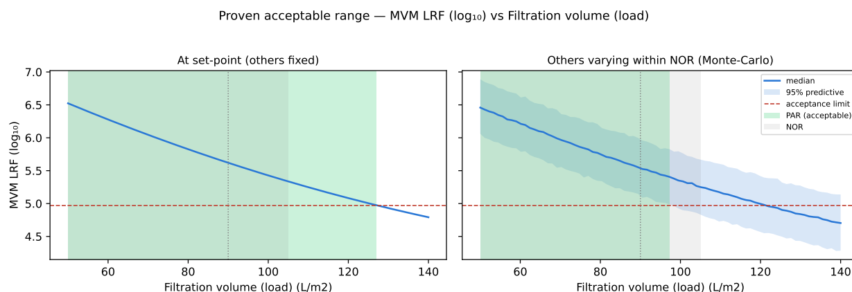
Figure 7.1: Proven acceptable range for MVM LRF against the filtration volume. The right panel propagates the filtration pressure across its normal operating range.
