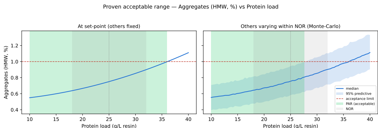
Figure 7.1: Proven acceptable range for pool aggregate against protein load, the parameter with the largest main effect on it.
