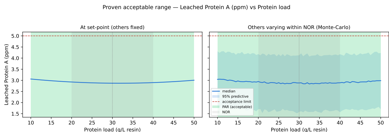
Figure 7.3: Proven acceptable range for leached Protein A against protein load, the parameter with the largest main effect on it.
