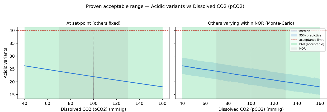
Figure 7.4: Proven acceptable range for acidic charge variants against its governing parameter.
