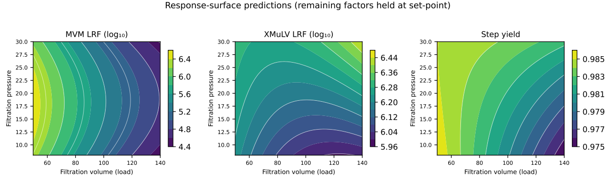
Figure 5.1: Response-surface predictions for MVM LRF, XMuLV LRF and step yield over the filtration volume and the filtration pressure.
