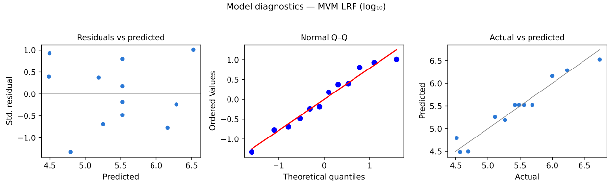
Figure 5.2: Model diagnostics for the MVM LRF response-surface model.
