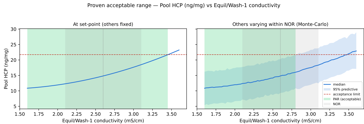
Figure 7.1: Proven acceptable range of the equilibration and wash-1 conductivity for pool host cell protein.
