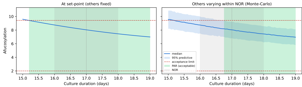
(a) Proven acceptable range for afucosylation against culture duration, at set-point and under normal operating range co-variation.
