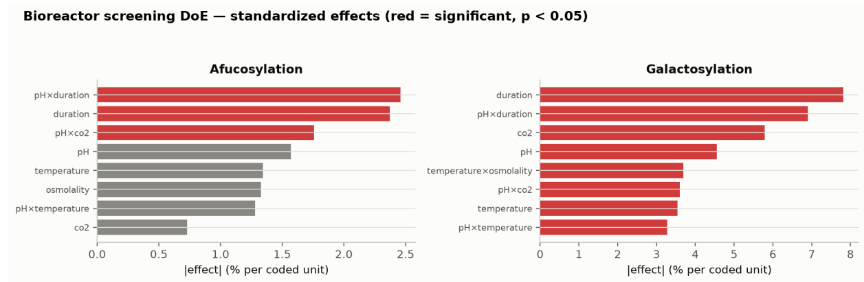
Figure 5.2: Standardized screening effects for afucosylation and galactosylation; red bars are significant ( p < 0.05 ).
