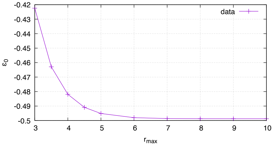
ground state energy \varepsilon_0 while sweeping over r_{\max}
