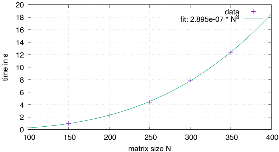
runtime of the decomposition algorithm
