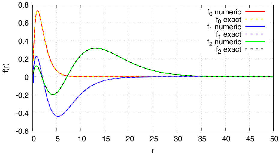
3 lowest reduced radial wavefunction
