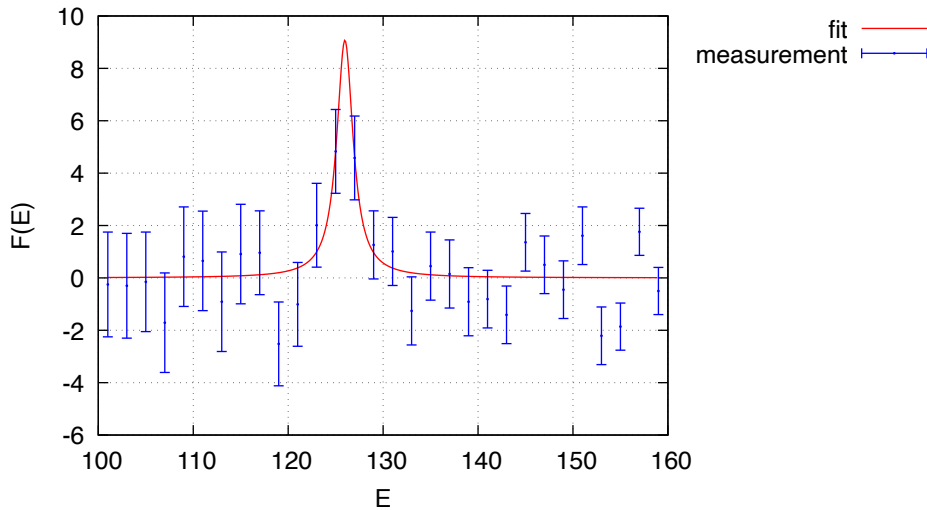
Fitted Breit Wigner function compared to the measurement
