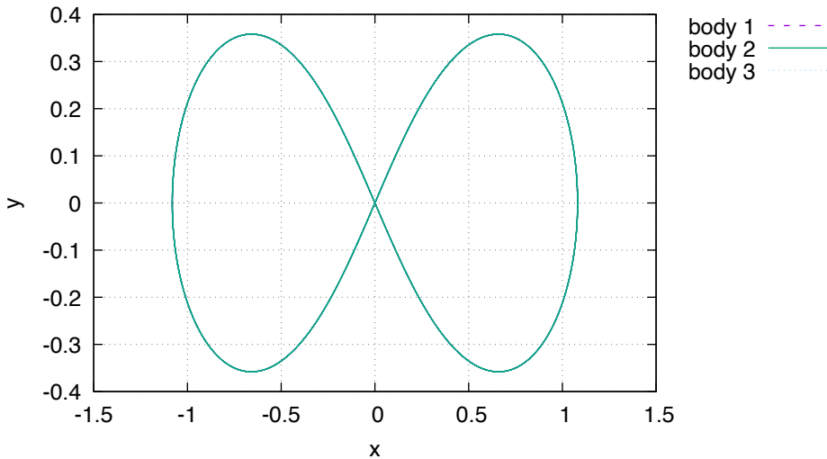
Solution of three-body problem
