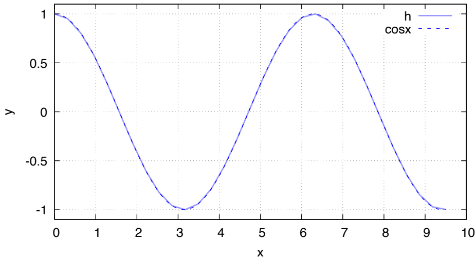
visualization of the quadratic spline(FS)
