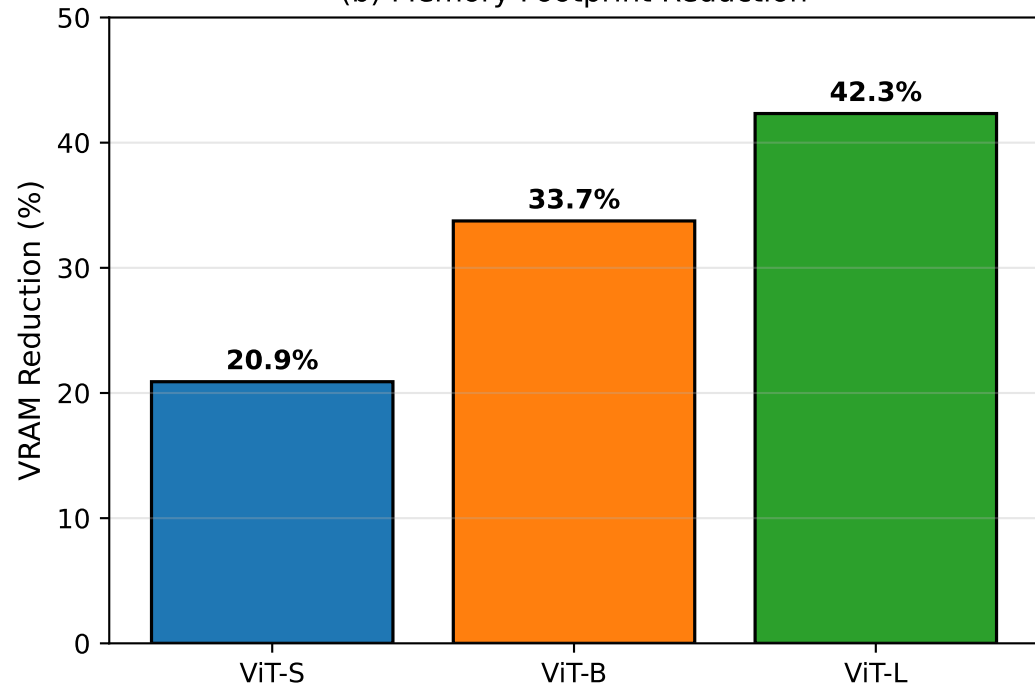
(b) Memory Footprint Reduction
