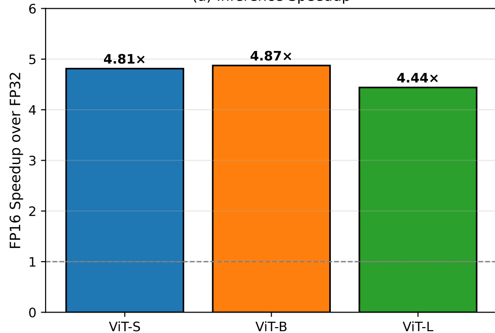
(a) Inference Speedup
