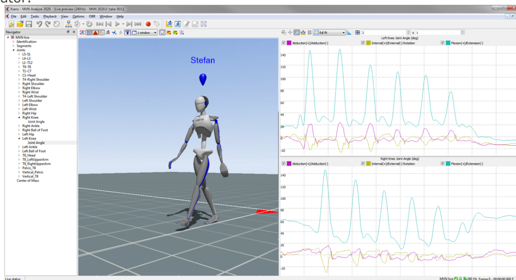
Figure 49: Real-time graphs
