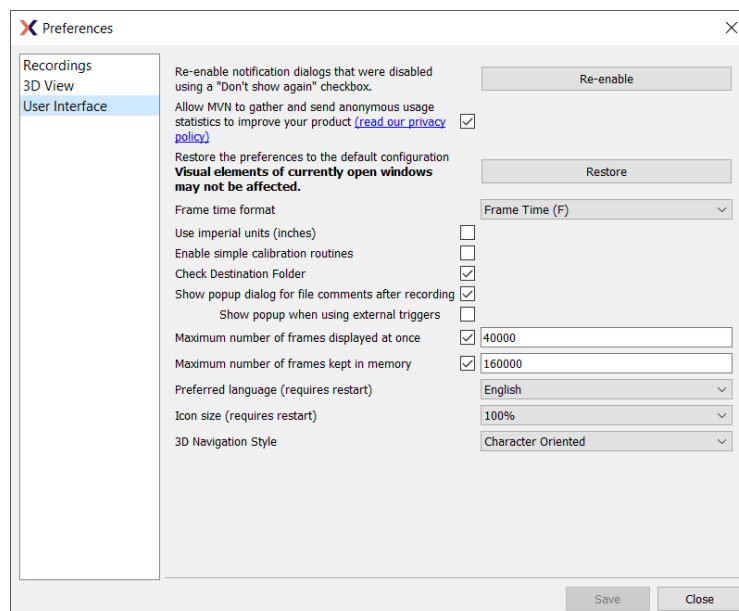
Figure 15: Preferences tab
