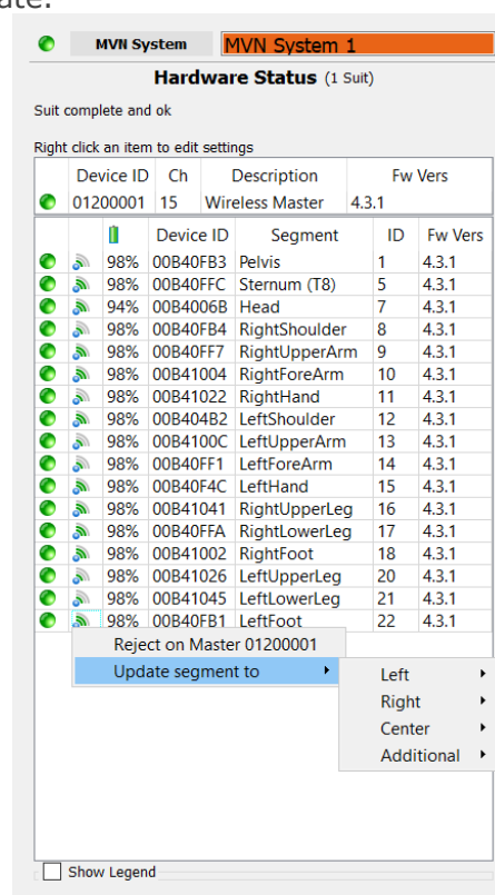
Figure 45 Relocating trackers
