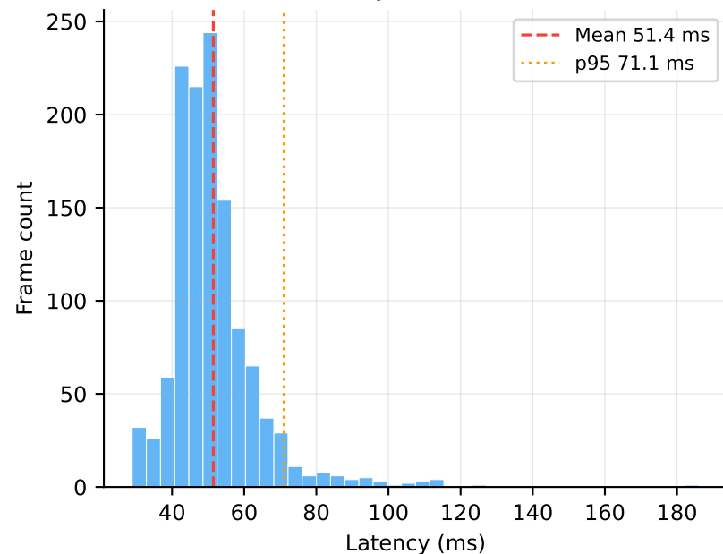
Latency Distribution
