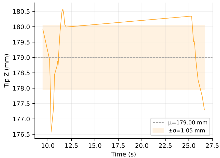
Tip Z (mm) vs Time
