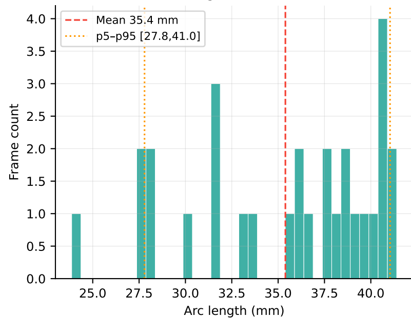
Arc Length Distribution
