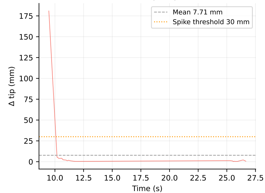
Frame-to-Frame Tip Displacement
