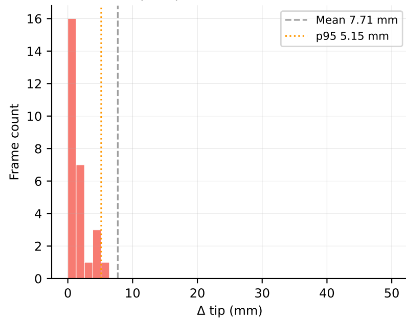
Tip Displacement Distribution
