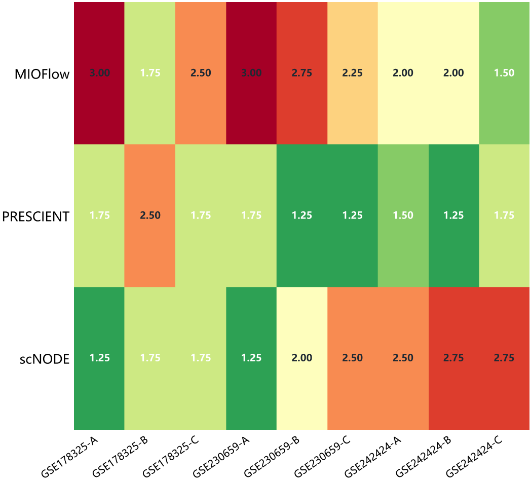
Forecast average rank
