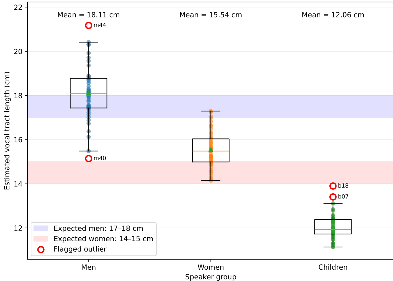
Estimated Vocal Tract Length by Speaker Group
