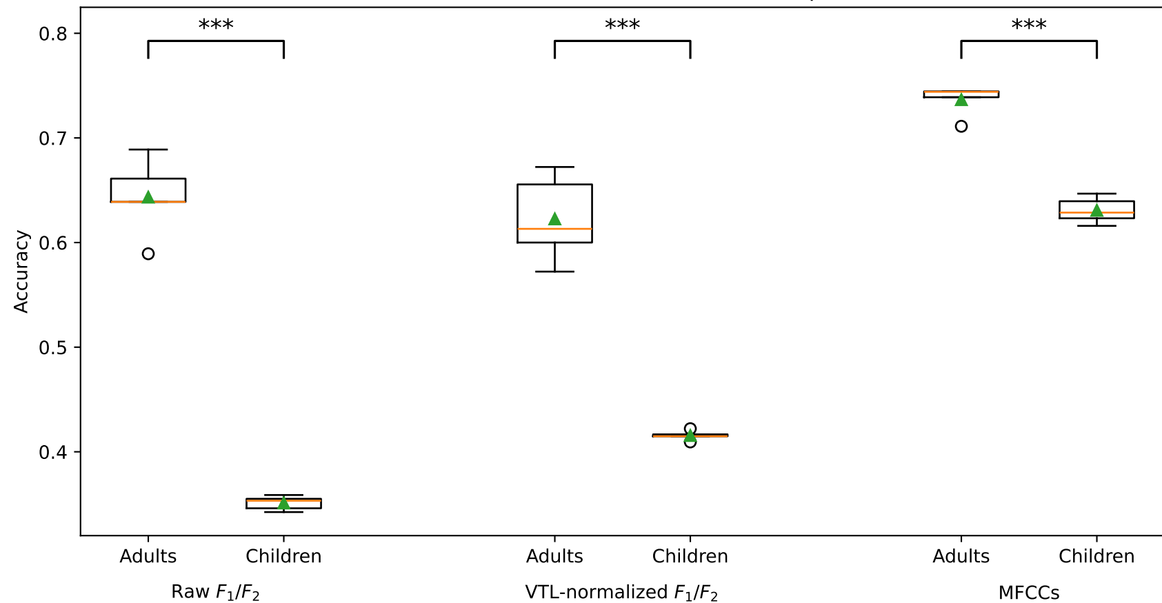
Adult-to-Child Generalization Across Feature Representations
