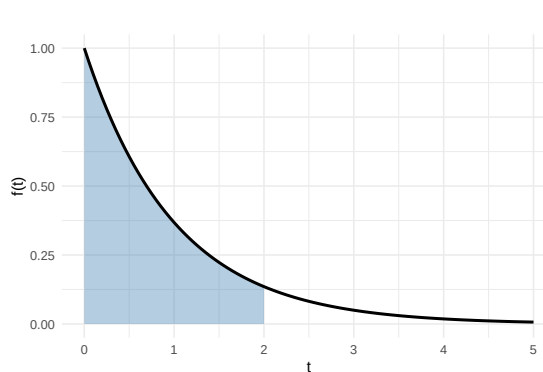
(a) PDF with \lambda = 1 ; shaded area equals F(2) \approx 0.865 .
