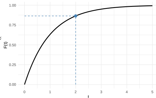
(b) CDF with \lambda = 1 ; point marks F(2) \approx 0.865 .
