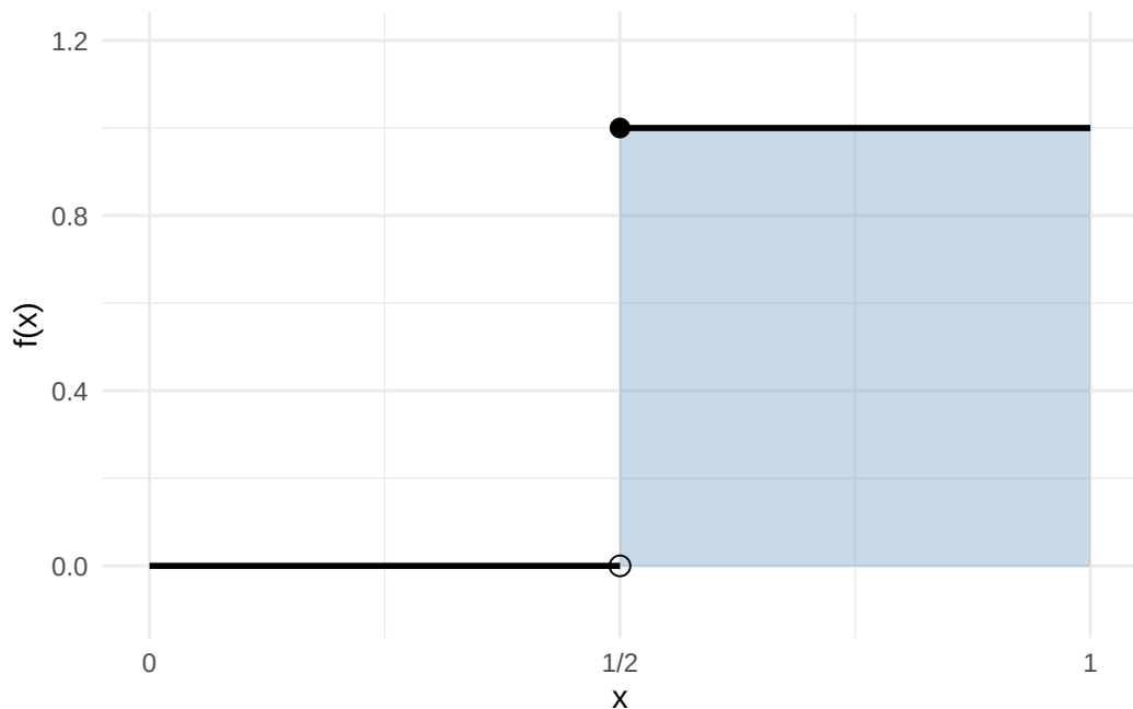
Figure 4: Step function: f(x) = 0 on [0, \frac{1}{2}) 47 (open circle at the jump) and f(x) = 1 on [\frac{1}{2}, 1] (filled circle). The shaded rectangle has area \frac{1}{2} , matching the integral computed in Example 0.32.
