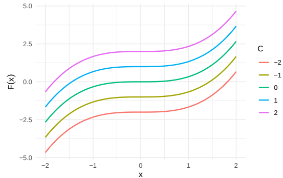
(b) Family of antiderivatives F(x) = x^3/3 + C .
