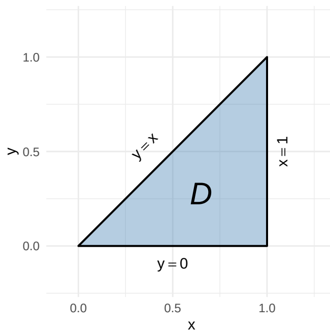
Figure 7: Triangular integration region D = \{(x, y) : x \in [0, 1], y \in [0, x]\} , bounded below by y = 0 , above-left by y = x , and on the right by x = 1 .
