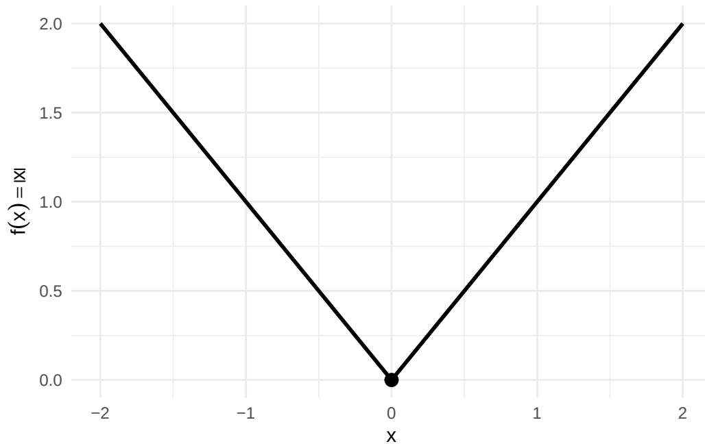
Figure 3: f(x) = |x| has a sharp corner at x = 0 (not differentiable there) but is continuous everywhere: no gaps or jumps.
