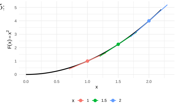
(b) F(x) = x^2 ; tangent slope at each marked x equals f(x) = 2x .
