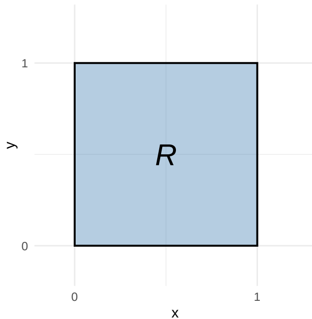
Figure 10: Integration region R = [0, 1]^2 , the unit square.
