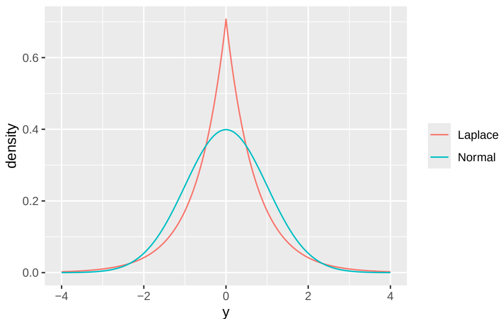
Figure 3: Laplace and standard normal densities with the same mean (0) and variance (1)
