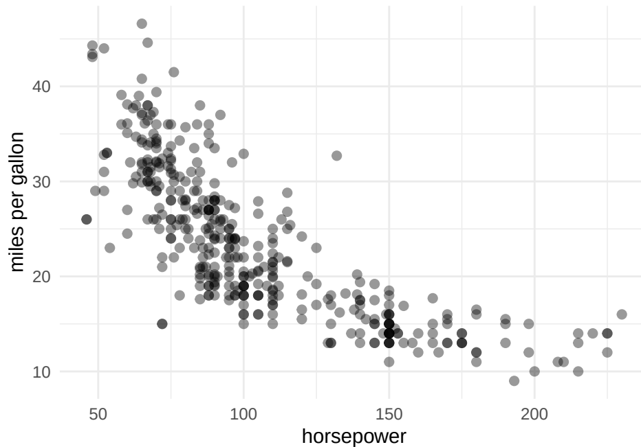
Figure 1: Miles per gallon against horsepower for the cars in the Auto data. Cars with more horsepower tend to have lower fuel economy.
