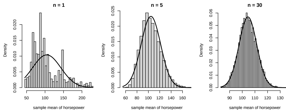
Figure 3: Histograms of 10,000 sample means of horsepower, for samples of n = 1, 5 and 30 cars drawn with replacement from the Auto data. The curve is the normal density with mean \mu and standard deviation \sigma/\sqrt{n} over the square root of n .
