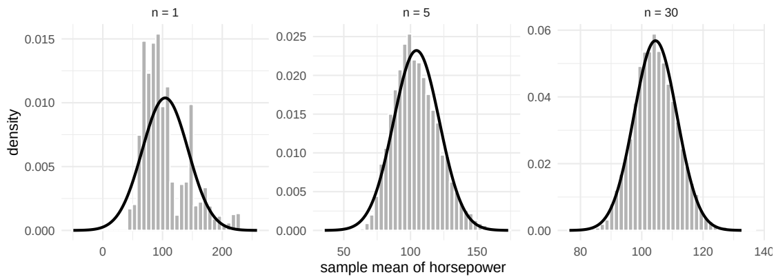
Figure 3: Histograms of 10,000 sample means of horsepower, for samples of n = 1 , 5 and 30 cars drawn with replacement from the Auto data. The curve is the normal density with mean \mu and standard deviation \sigma/\sqrt{n} over the square root of n .
