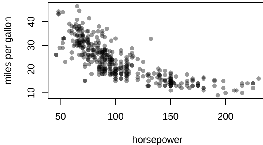
Figure 1: Miles per gallon against horsepower for the cars in the Auto data. Cars with more horsepower tend to have lower fuel economy.
