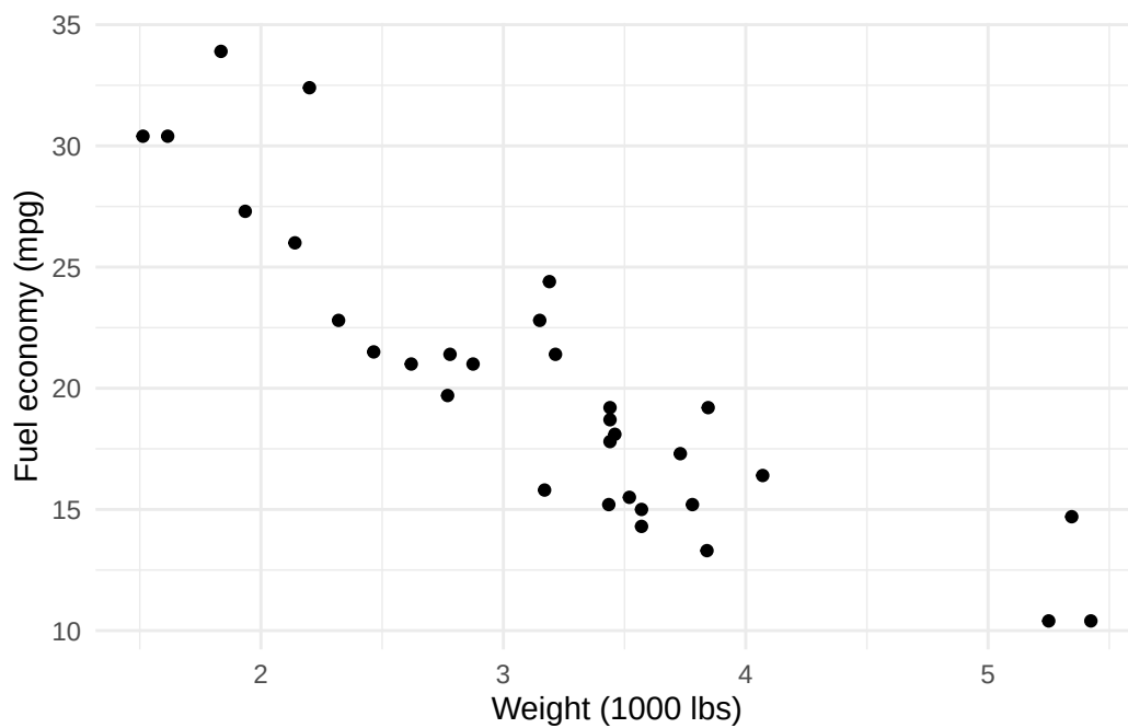
Figure 1: Fuel economy vs. weight for 32 cars.
